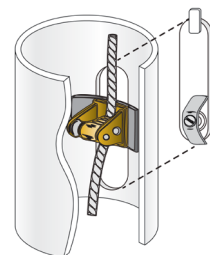
Internal Cam Cleat & Handhole Door
